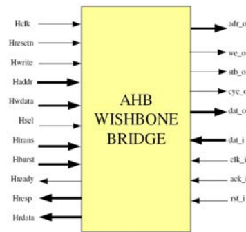
Figure 1: The AHB-2-Wishbone bridge – an OpenCores design
